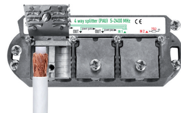
Insertion of the inner conductor into the hole
