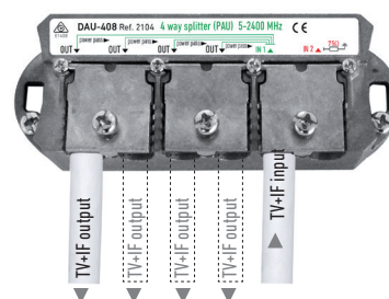
Connection for an installation DAU splitter mode
