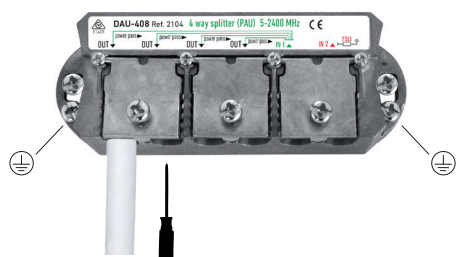
Closing of the flange cover by means of the screw
