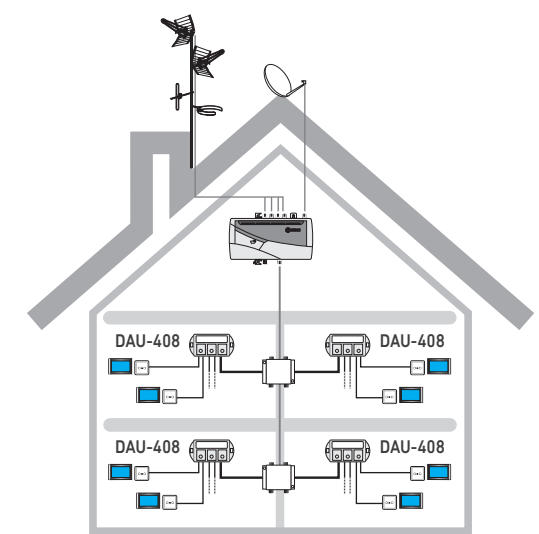
Application example (splitter mode)
